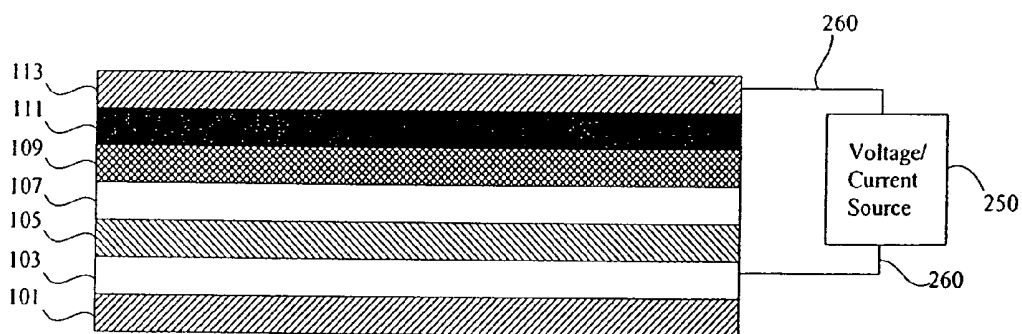
Figure 9 (Prior Art)
